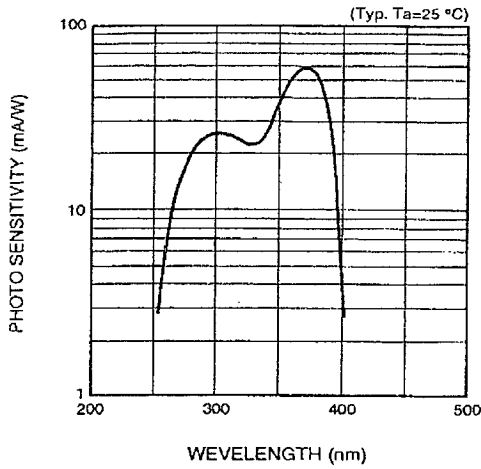
Figure 1: Spectral Response
